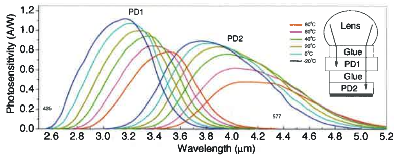
Fig. 1. Photoresponse spectra of the dual band photodiode with InAs (PD1) and InAsSb (PD2) active layers at several photodiode temperatures. In the insert – schematic of the device (RF patent application# 2013109254).
