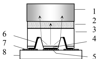
Fig.1 Scheme of a "fibre" LED, 1- optical fibre, 2- optical "glue" –chalcogenide glass ( n=2.4 ), 3- transparent substrate or "broad band window", 4- active zone of the device (p-n junction) 5- anode connected with bonding area, 6-gold contacts ( cathodes), 7- alloy – bonding areas, 8- semiinsulating silicon submount (header)
