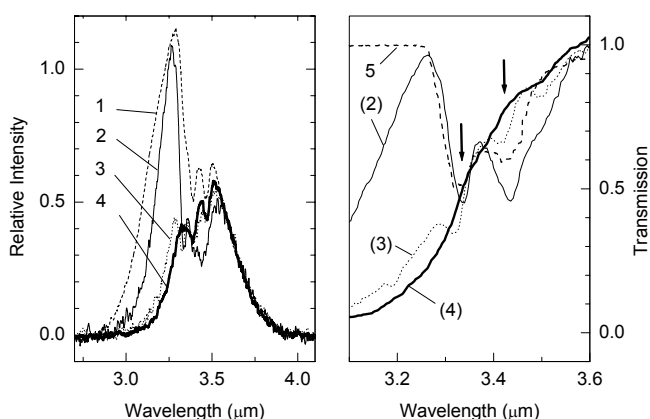
Fig.2 Emission of the 3.4 \mu\text{m} LED coupled with 15-cm long fibre measured at the end of the latter at the presence of air (1), alcohol (2), vodka (3) and water (4) ( all at the left) and the corresponding transmission of the fiber/evanescent wave.(right) (5) – direct measurements of the alcohol vapor transmission in a 10 cm long gas cell
