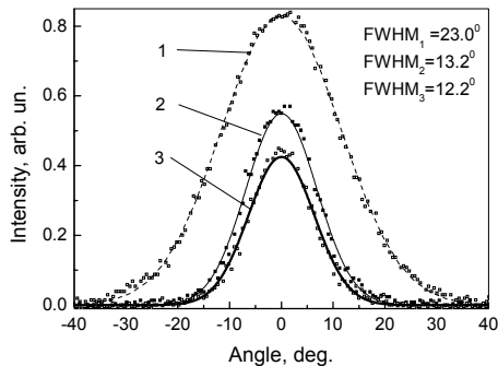
Fig.3 Far field pattern of the 3.4 \mu\text{m} radiation coming from the end of the fiber merged into alcohol (2) and vodka (3), (1) – initial pattern of the radiation (without liquid)
